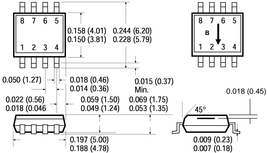
Fig. 3 Package information and magnetic sensitive direction
