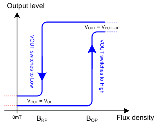
Fig.2 – Inverted South Active Pole
