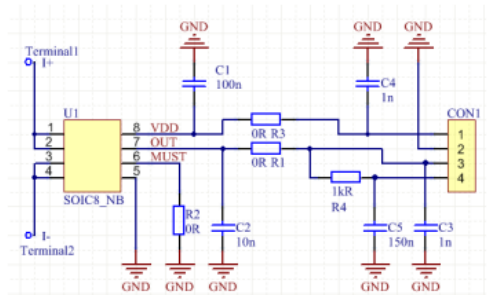
PCB schematic
